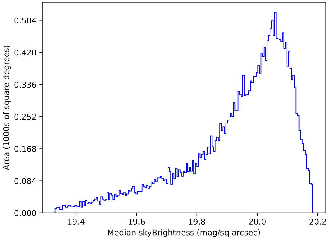
too_combined_s0.5_v3.4_10yrs All sky i band: Median skyBrightness
