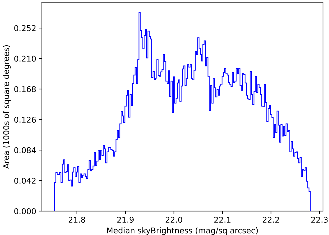
too_combined_s0.5_v3.4_10yrs All sky g band: Median skyBrightness
