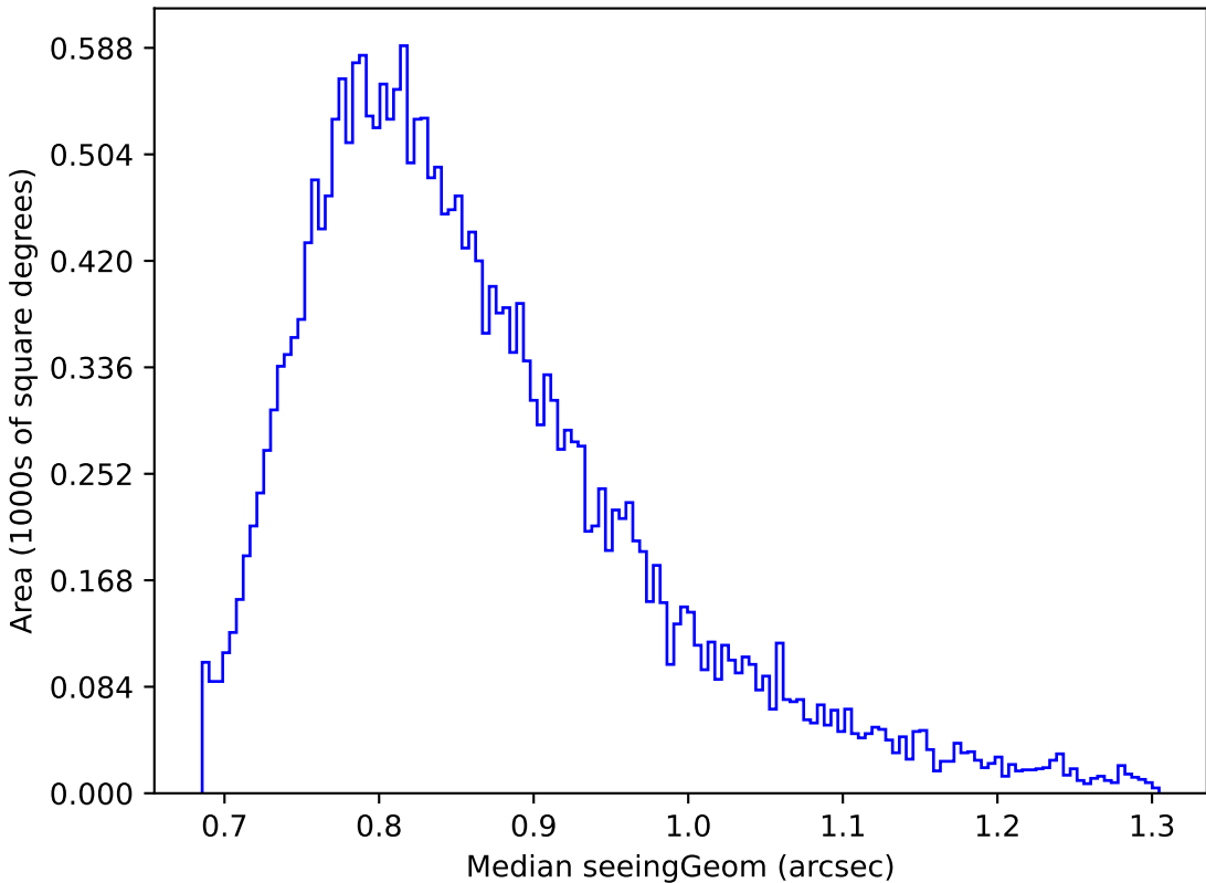
too_combined_s0.5_v3.4_10yrs Yr 1 z band: Median seeingGeom
