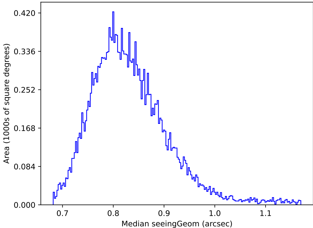
too_combined_s0.5_v3.4_10yrs Yr 1 y band: Median seeingGeom
