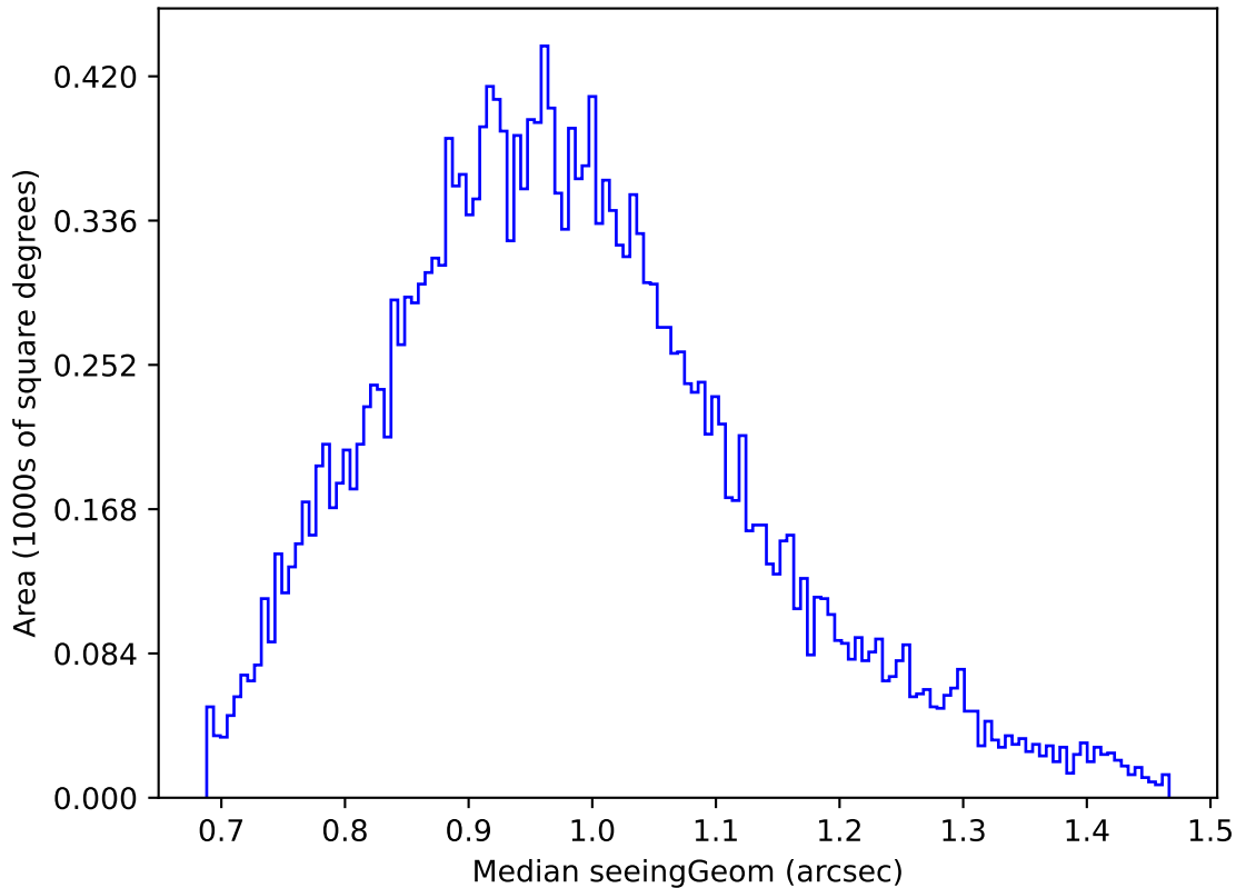
too_combined_s0.5_v3.4_10yrs Yr 1 u band: Median seeingGeom
