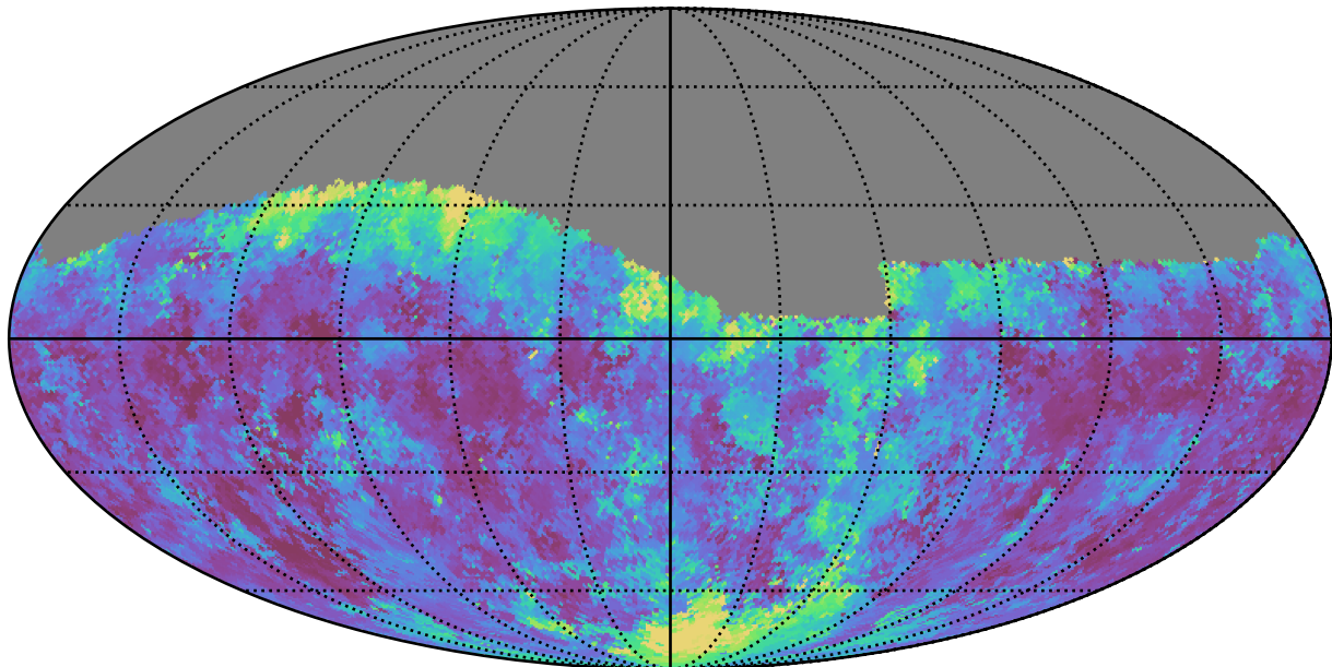
too_combined_s0.5_v3.4_10yrs Yr 1 g band: Median seeingGeom
