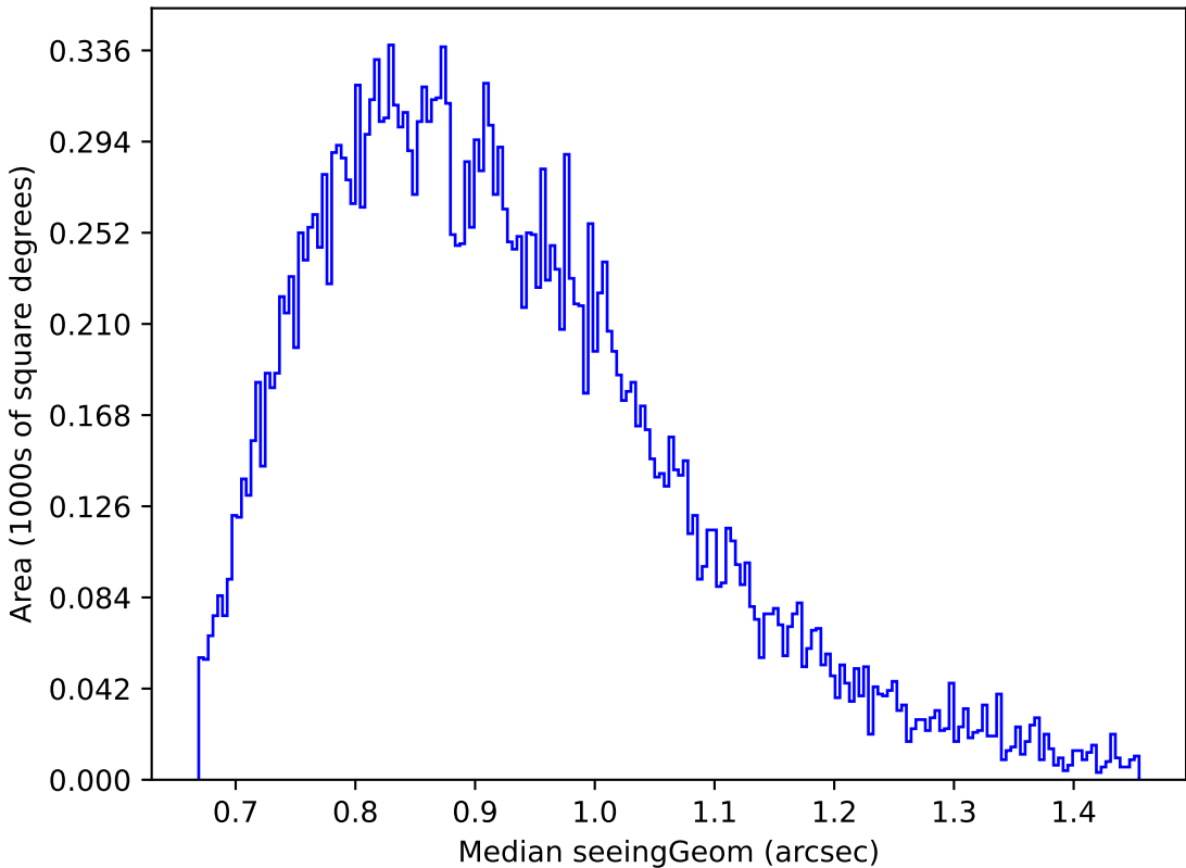
too_combined_s0.5_v3.4_10yrs Yr 1 g band: Median seeingGeom
