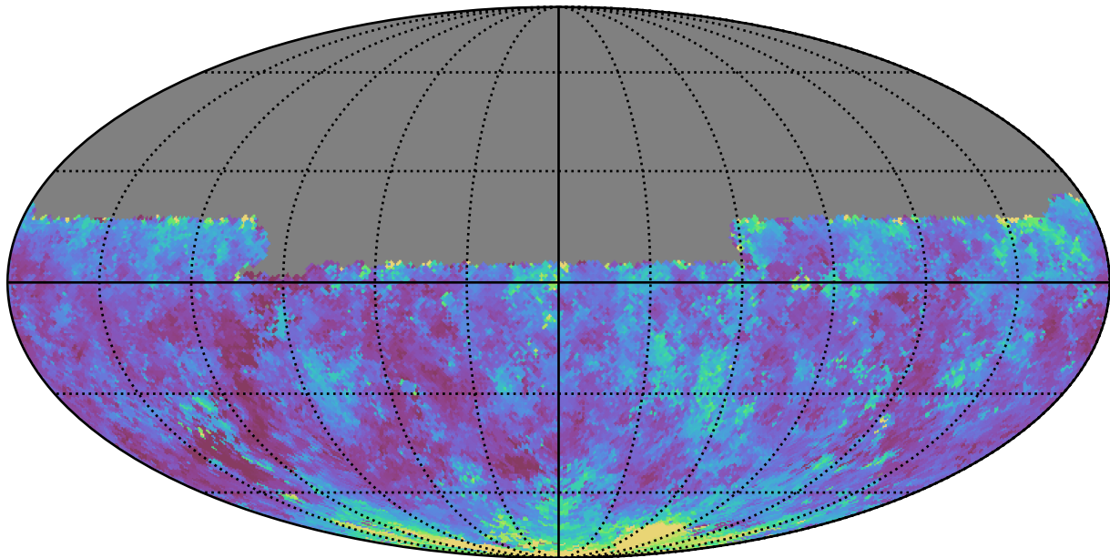
too_combined_s0.5_v3.4_10yrs Yr 1 y band: Median seeingEff
