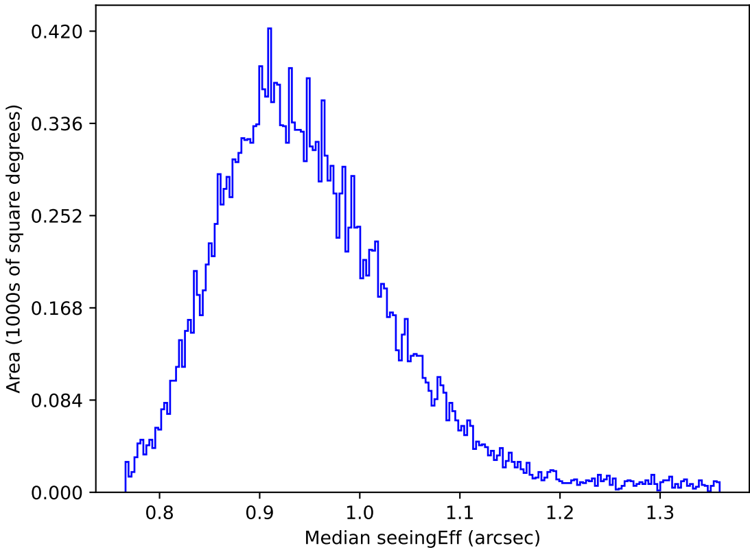
too_combined_s0.5_v3.4_10yrs Yr 1 y band: Median seeingEff
