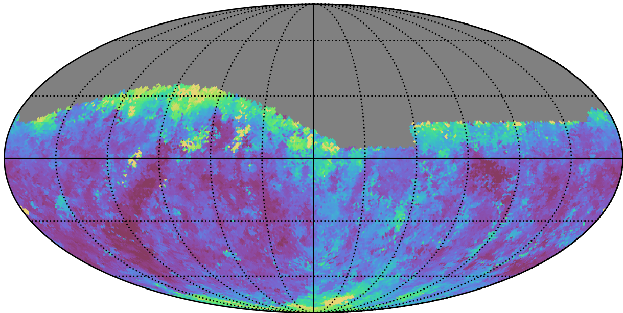
too_combined_s0.5_v3.4_10yrs Yr 1 r band: Median seeingEff
