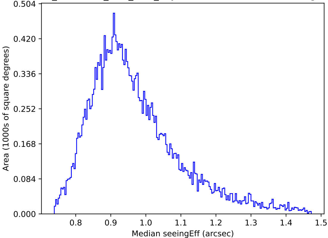
too_combined_s0.5_v3.4_10yrs Yr 1 r band: Median seeingEff
