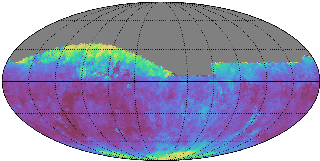
too_combined_s0.5_v3.4_10yrs Yr 1 all bands: Median seeingEff
