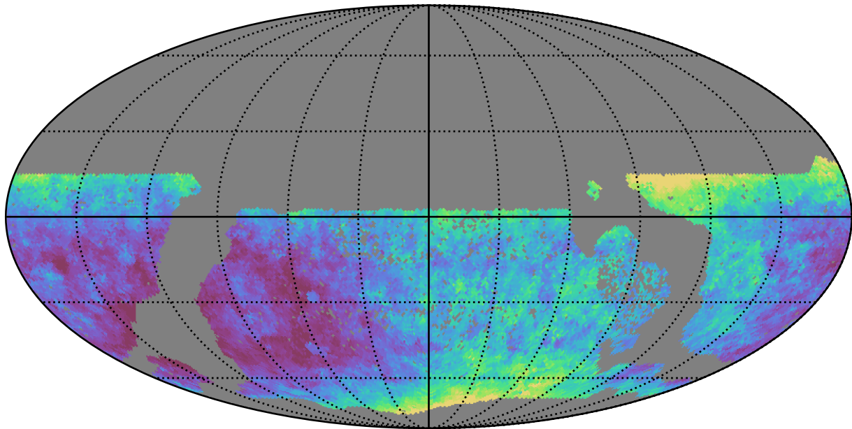
too_combined_s0.5_v3.4_10yrs WFD z band: Median seeingEff
