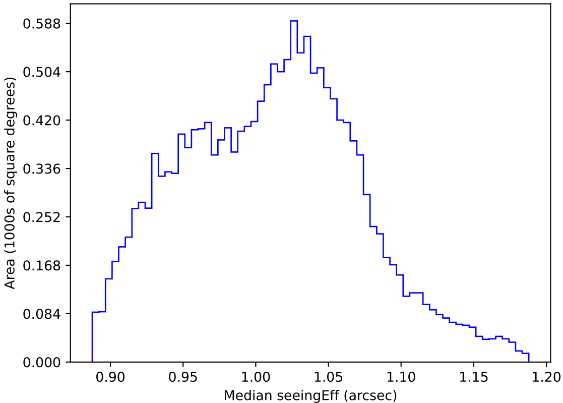
too_combined_s0.5_v3.4_10yrs WFD z band: Median seeingEff
