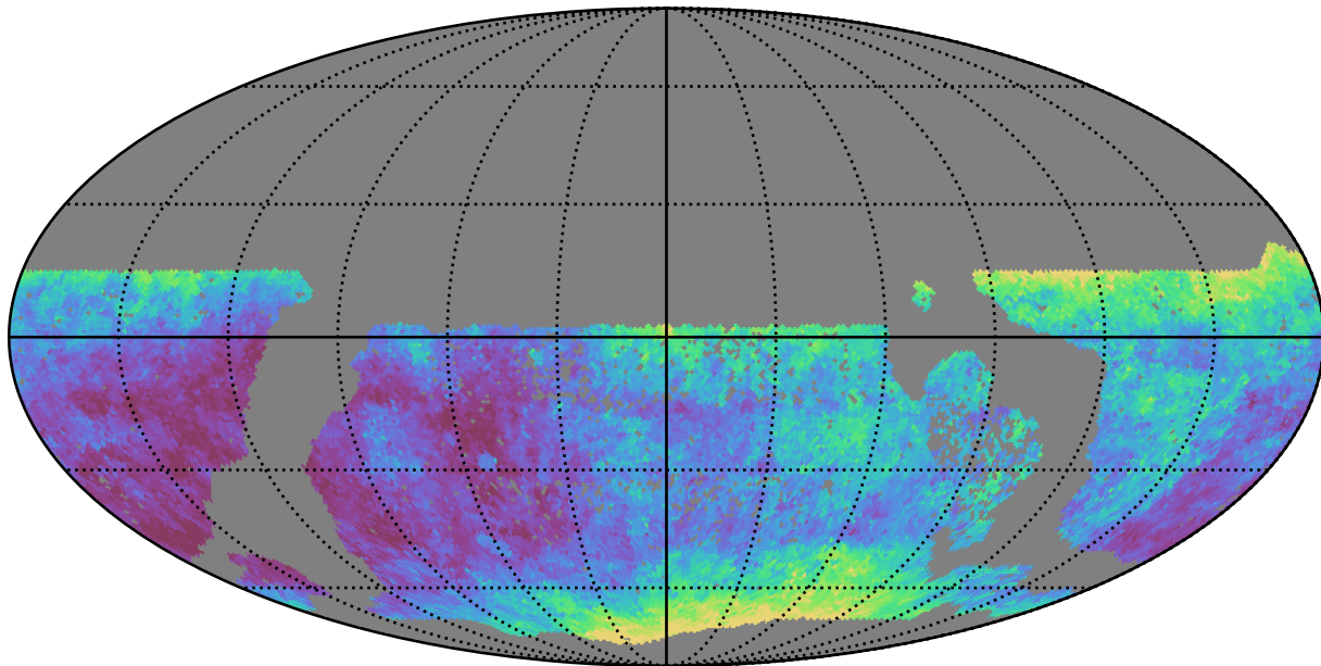
too_combined_s0.5_v3.4_10yrs WFD y band: Median seeingEff
