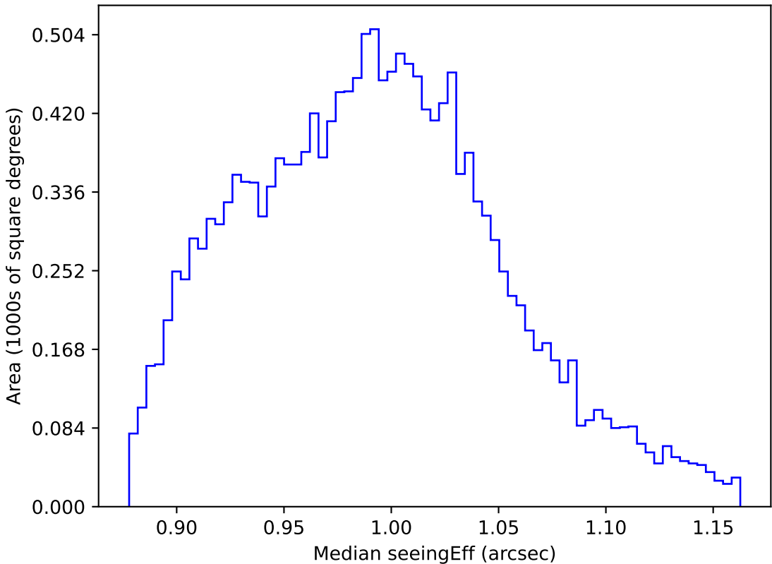
too_combined_s0.5_v3.4_10yrs WFD y band: Median seeingEff
