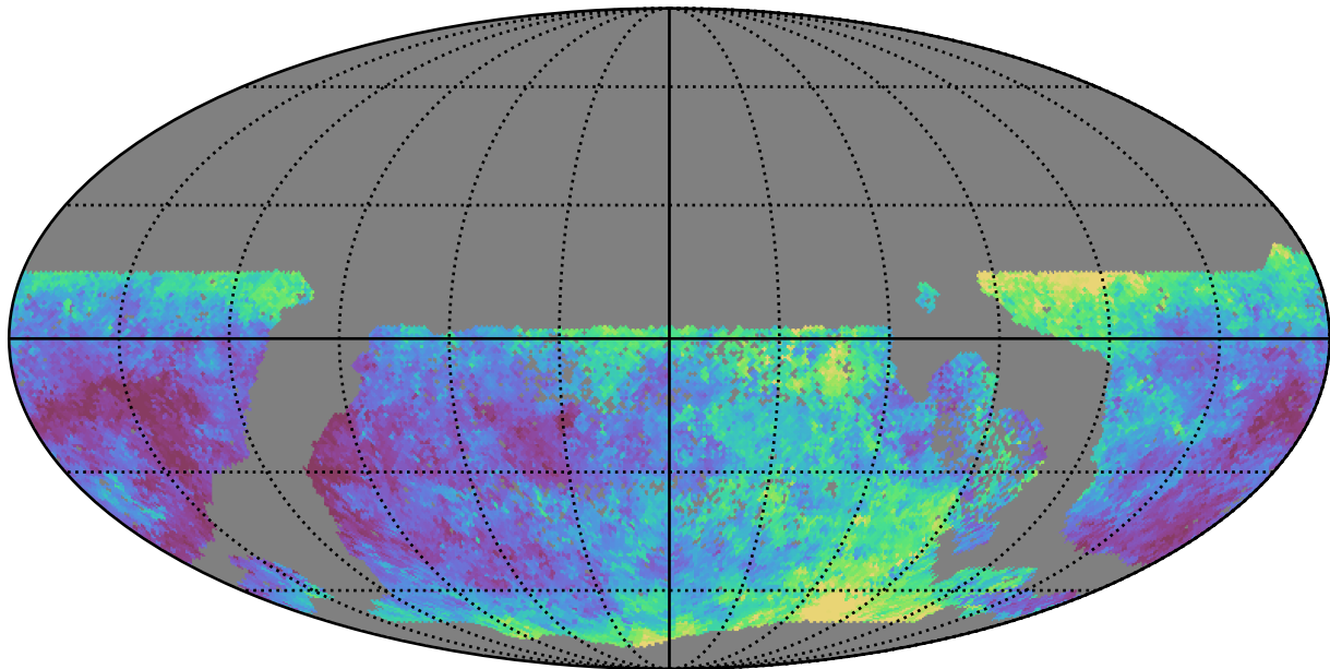
too_combined_s0.5_v3.4_10yrs WFD u band: Median seeingEff
