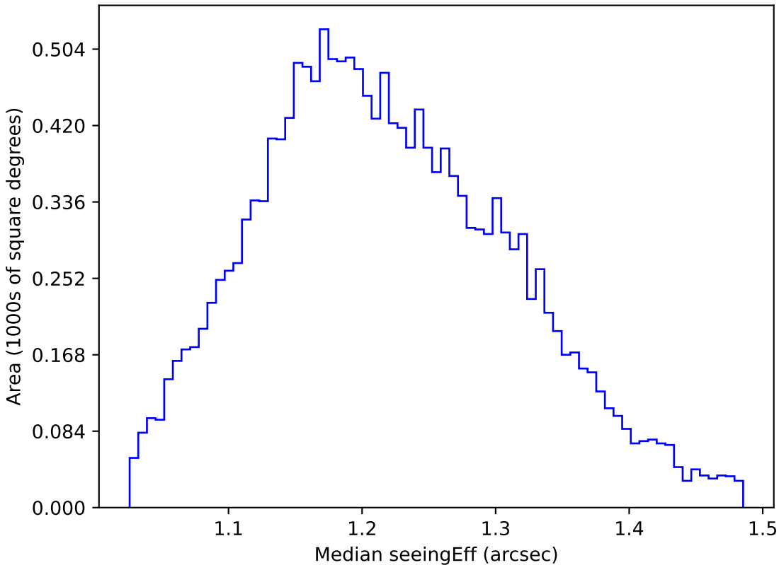
too_combined_s0.5_v3.4_10yrs WFD u band: Median seeingEff
