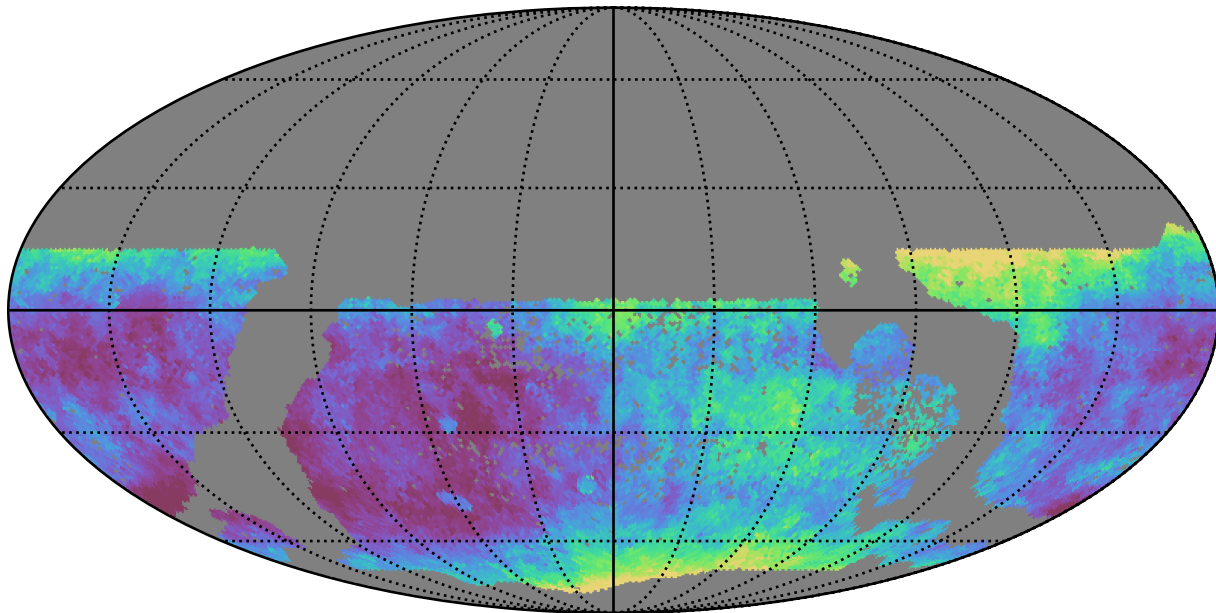
too_combined_s0.5_v3.4_10yrs WFD r band: Median seeingEff
