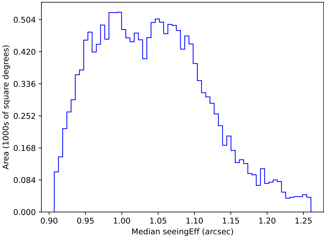
too_combined_s0.5_v3.4_10yrs WFD r band: Median seeingEff
