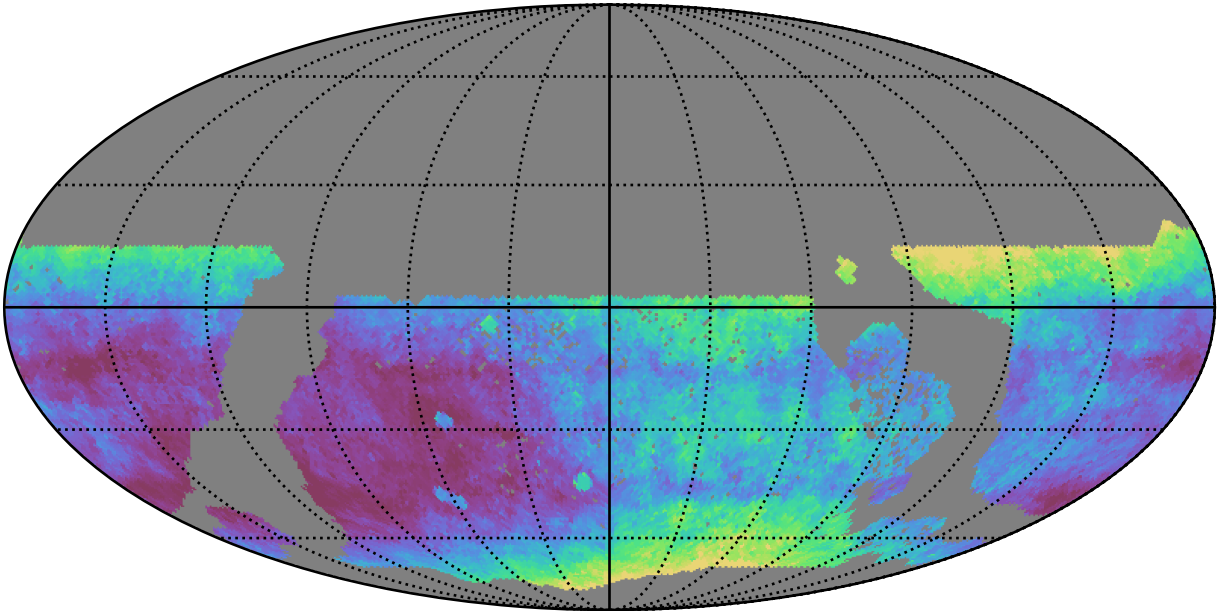
too_combined_s0.5_v3.4_10yrs WFD i band: Median seeingEff
