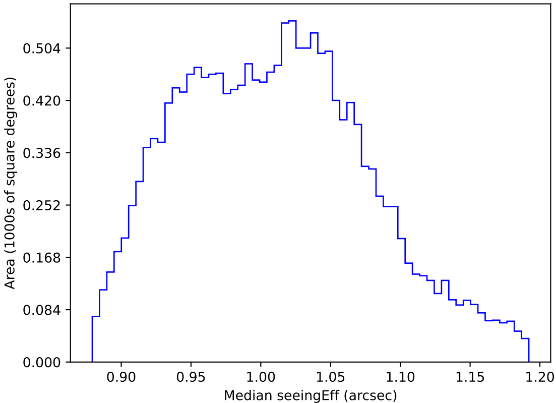
too_combined_s0.5_v3.4_10yrs WFD i band: Median seeingEff
