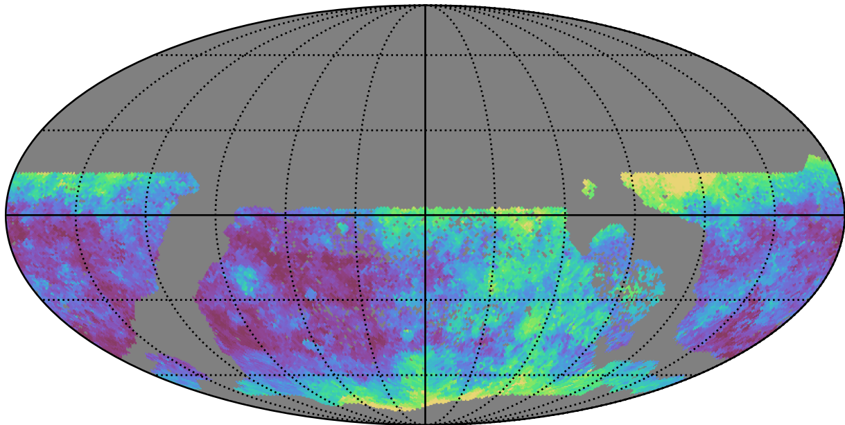
too_combined_s0.5_v3.4_10yrs WFD g band: Median seeingEff
