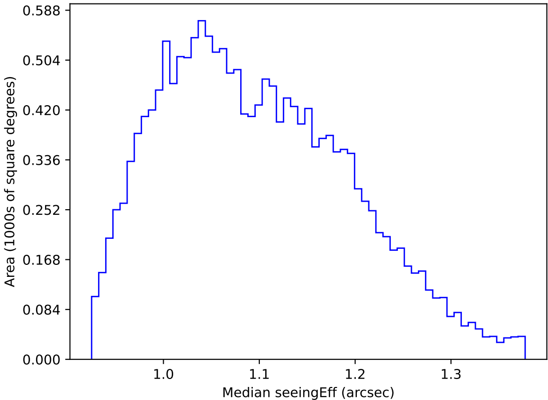
too_combined_s0.5_v3.4_10yrs WFD g band: Median seeingEff
