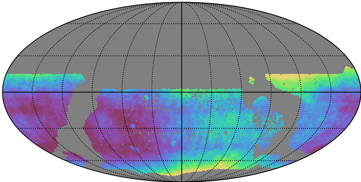
too_combined_s0.5_v3.4_10yrs WFD all bands: Median seeingEff
