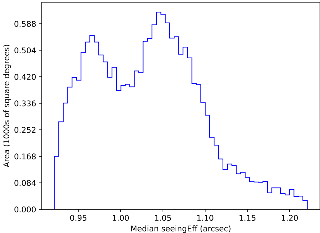
too_combined_s0.5_v3.4_10yrs WFD all bands: Median seeingEff
