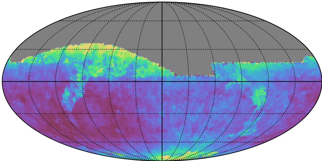
too_combined_s0.5_v3.4_10yrs All sky z band: Median seeingEff
