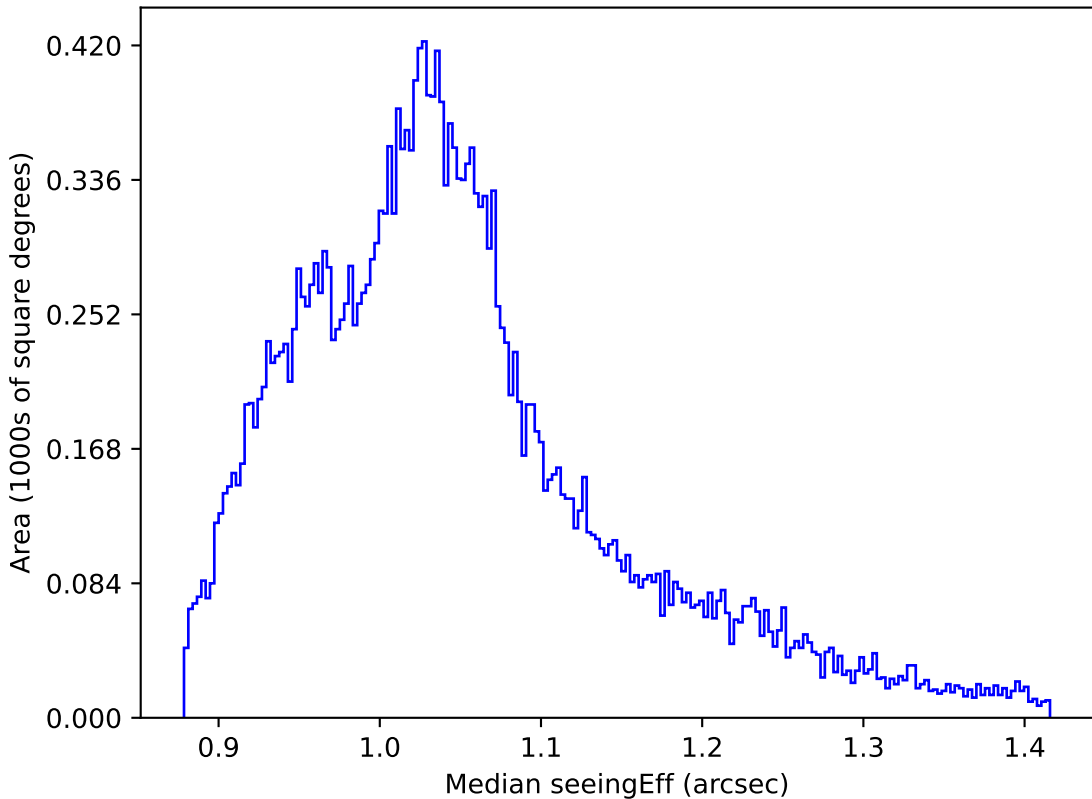
too_combined_s0.5_v3.4_10yrs All sky z band: Median seeingEff
