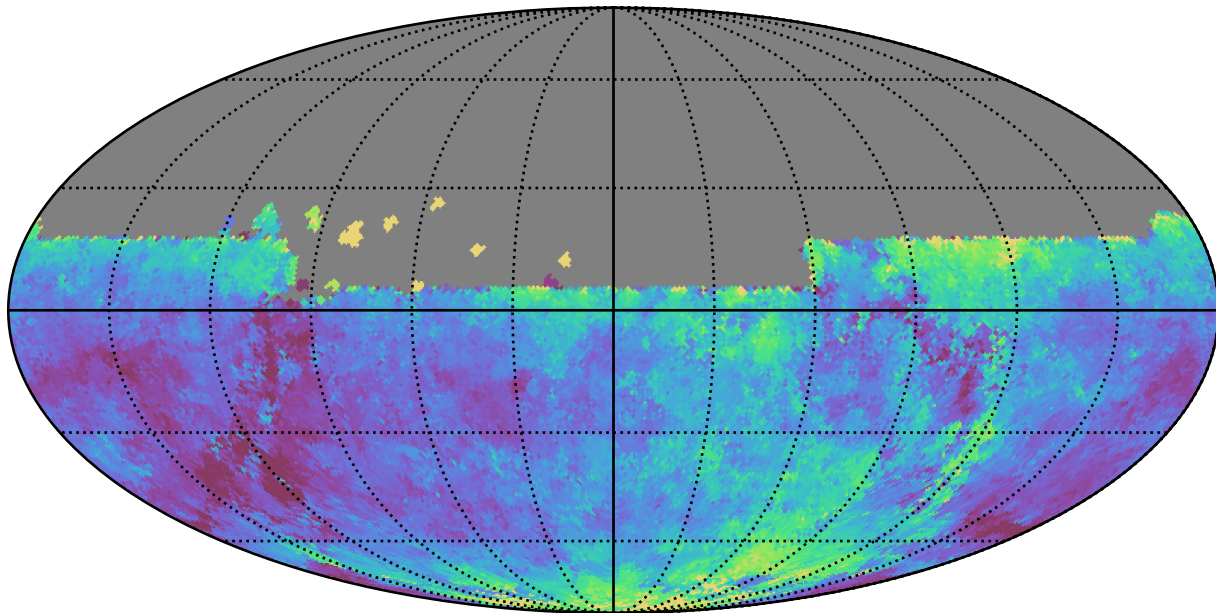
too_combined_s0.5_v3.4_10yrs All sky u band: Median seeingEff
