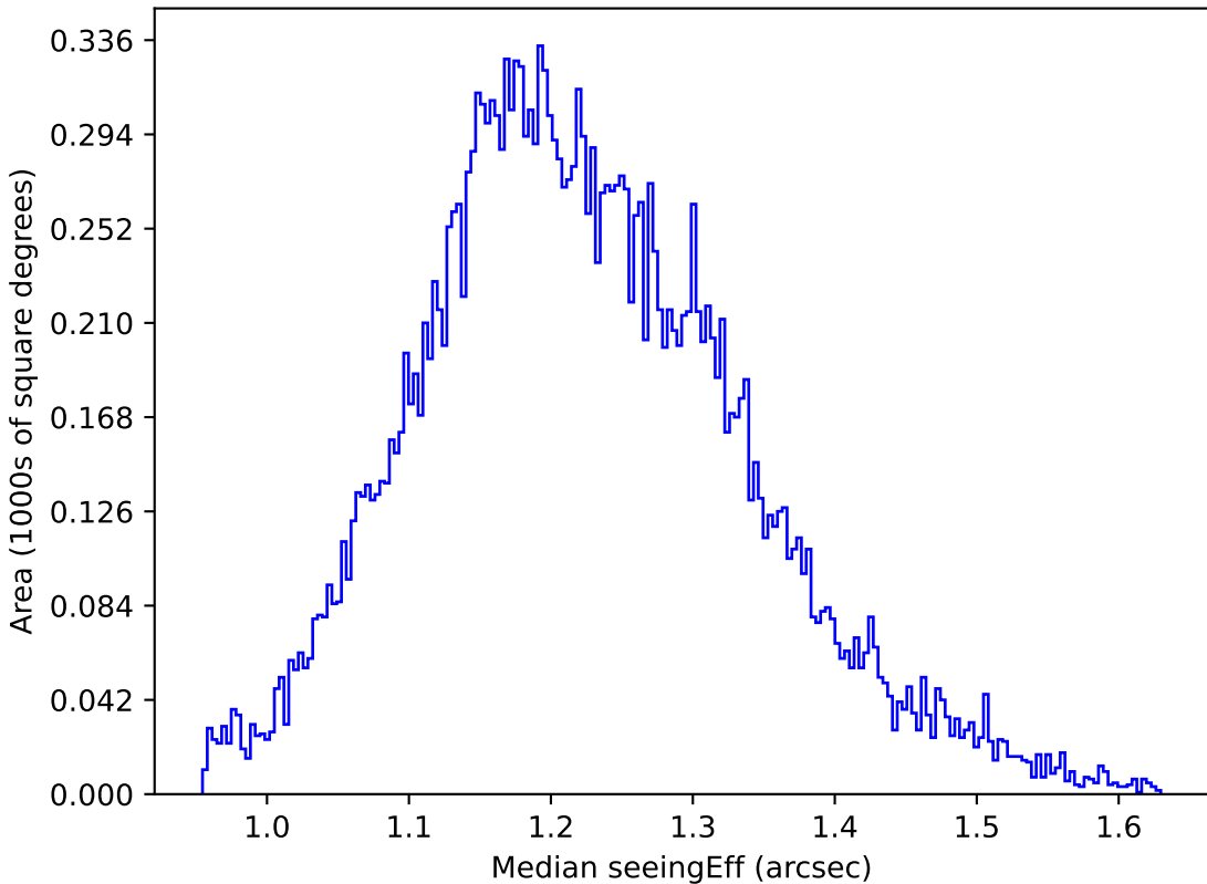
too_combined_s0.5_v3.4_10yrs All sky u band: Median seeingEff
