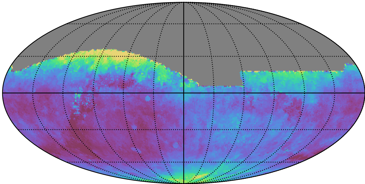
too_combined_s0.5_v3.4_10yrs All sky r band: Median seeingEff
