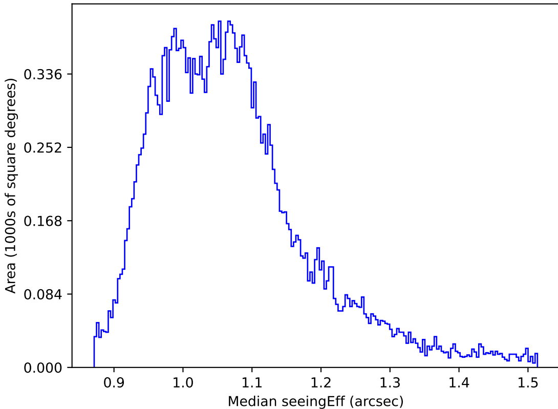
too_combined_s0.5_v3.4_10yrs All sky r band: Median seeingEff
