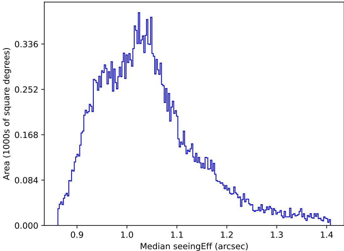
too_combined_s0.5_v3.4_10yrs All sky i band: Median seeingEff
