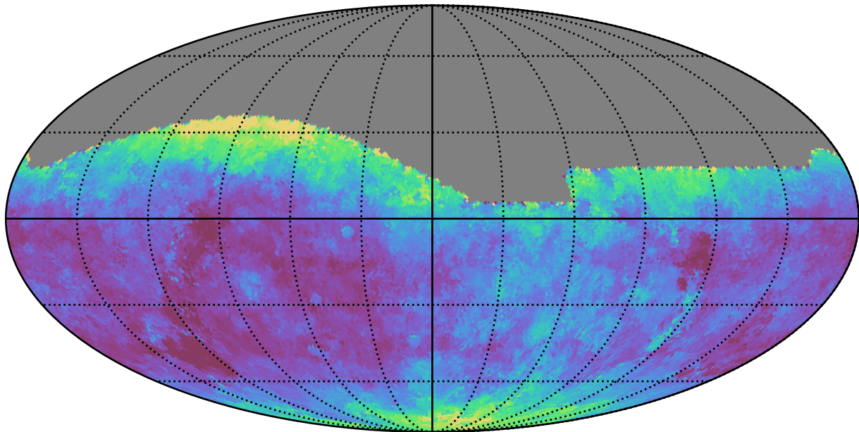
too_combined_s0.5_v3.4_10yrs All sky g band: Median seeingEff
