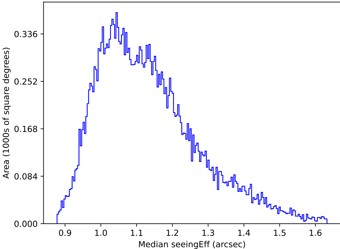
too_combined_s0.5_v3.4_10yrs All sky g band: Median seeingEff
