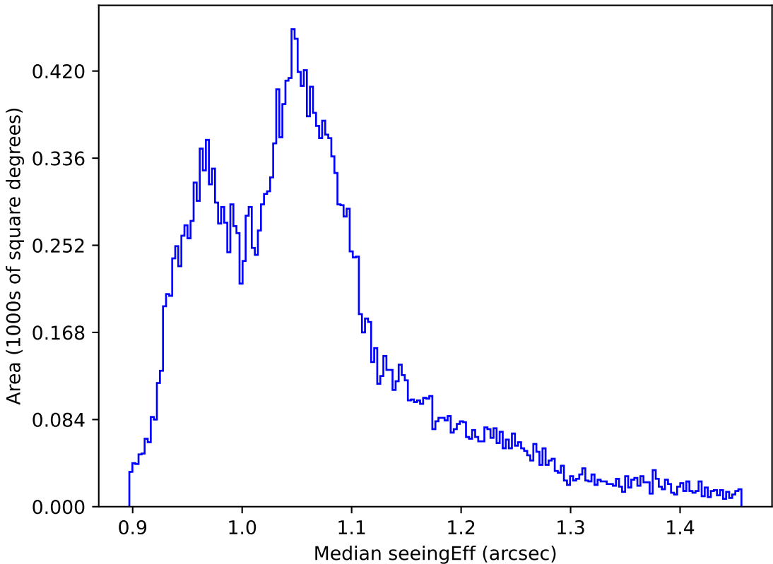
too_combined_s0.5_v3.4_10yrs All sky all bands: Median seeingEff
