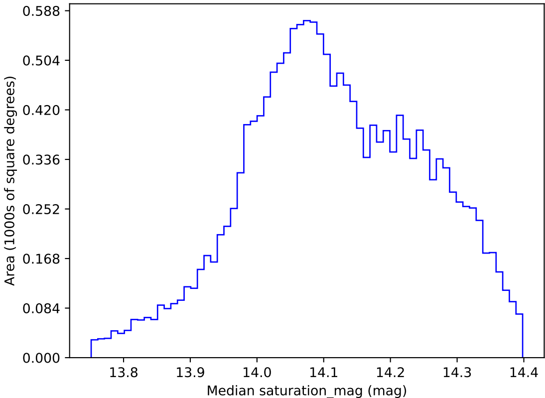
too_combined_s0.5_v3.4_10yrs WFD z band: Median saturation_mag
