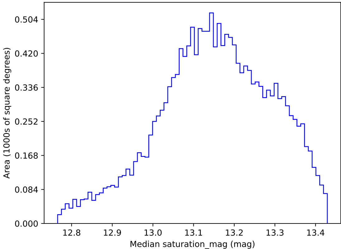
too_combined_s0.5_v3.4_10yrs WFD y band: Median saturation_mag
