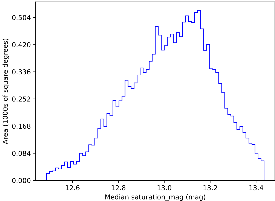
too_combined_s0.5_v3.4_10yrs WFD u band: Median saturation_mag
