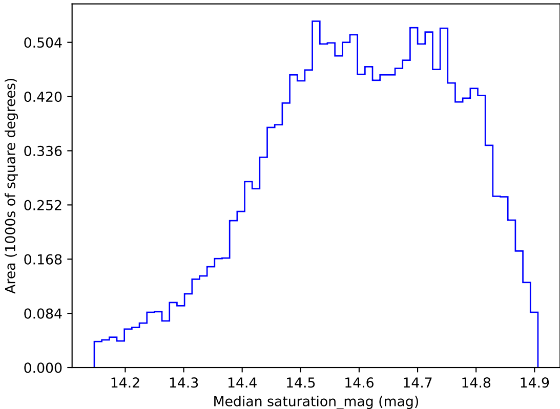
too_combined_s0.5_v3.4_10yrs WFD r band: Median saturation_mag
