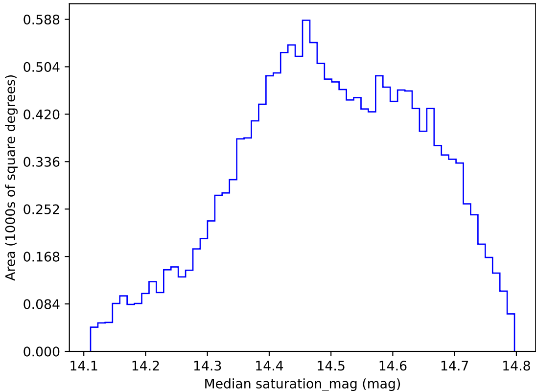
too_combined_s0.5_v3.4_10yrs WFD i band: Median saturation_mag
