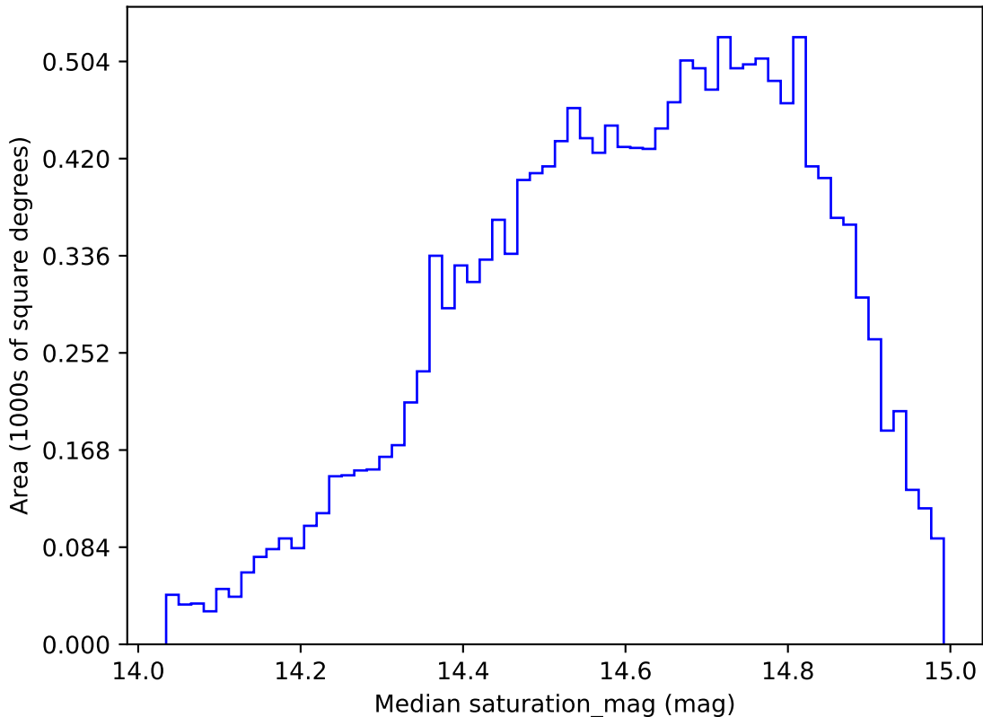
too_combined_s0.5_v3.4_10yrs WFD g band: Median saturation_mag
