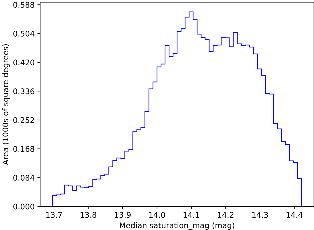
too_combined_s0.5_v3.4_10yrs WFD all bands: Median saturation_mag
