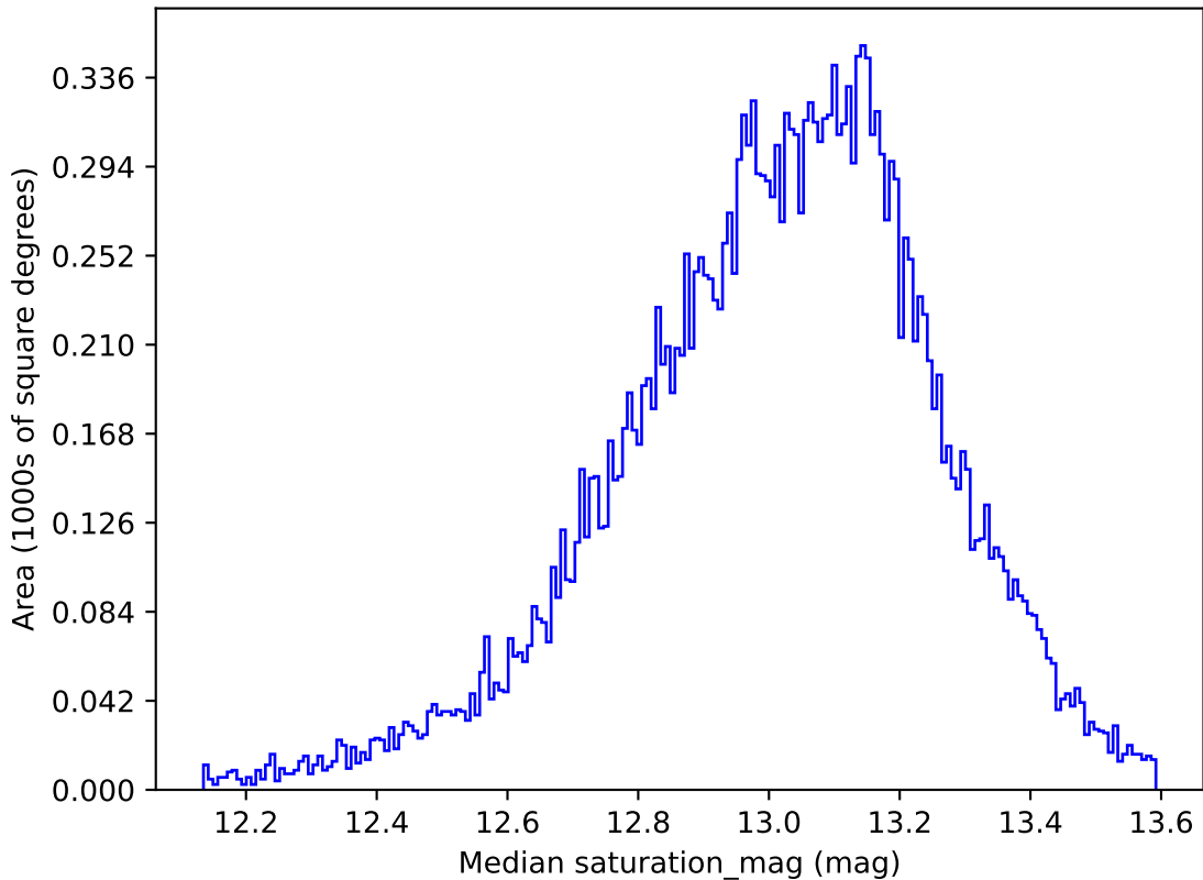
too_combined_s0.5_v3.4_10yrs All sky u band: Median saturation_mag
