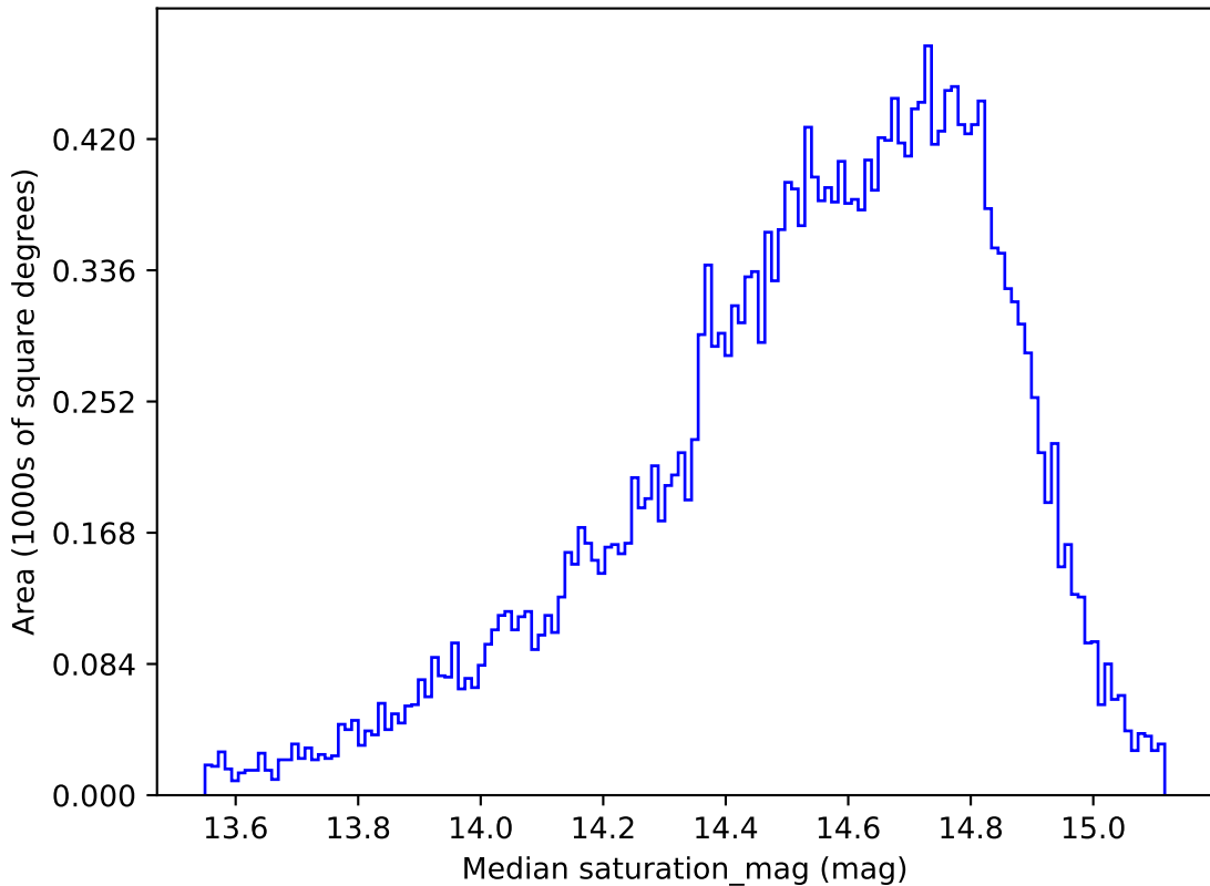
too_combined_s0.5_v3.4_10yrs All sky g band: Median saturation_mag
