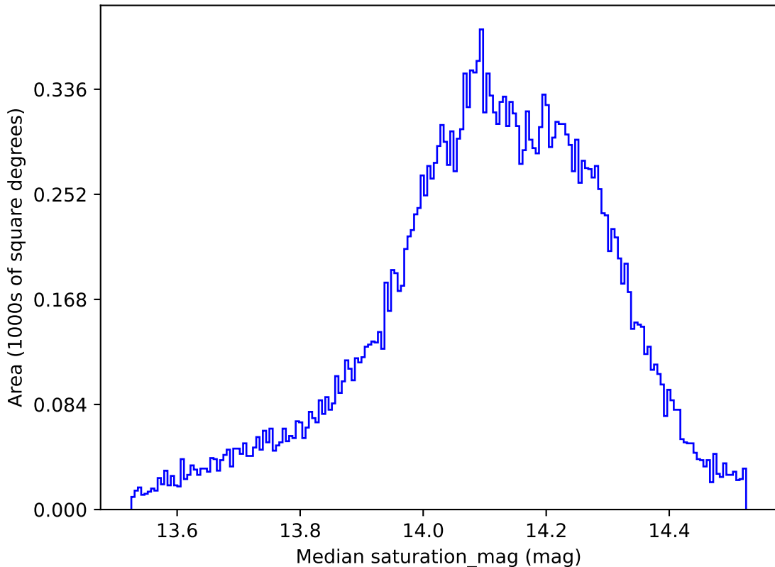
too_combined_s0.5_v3.4_10yrs All sky all bands: Median saturation_mag
