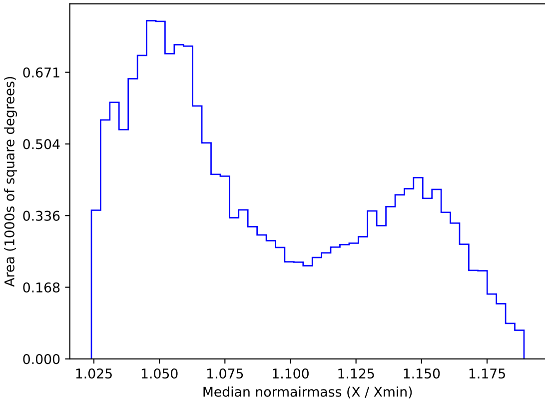
too_combined_s0.5_v3.4_10yrs WFD z band: Median normairmass
