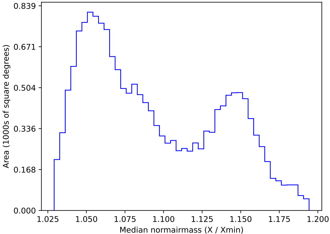
too_combined_s0.5_v3.4_10yrs WFD y band: Median normairmass
