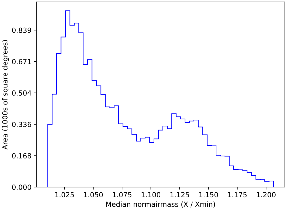
too_combined_s0.5_v3.4_10yrs WFD u band: Median normairmass
