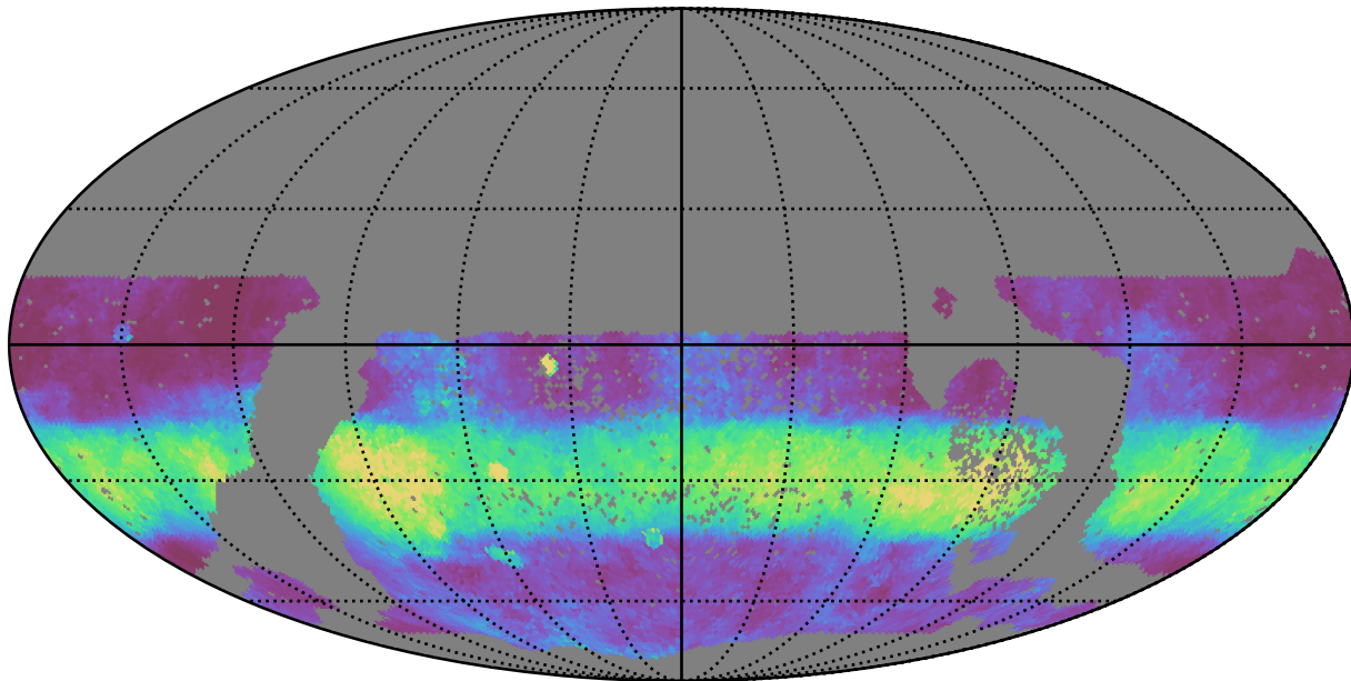
too_combined_s0.5_v3.4_10yrs WFD r band: Median normairmass
